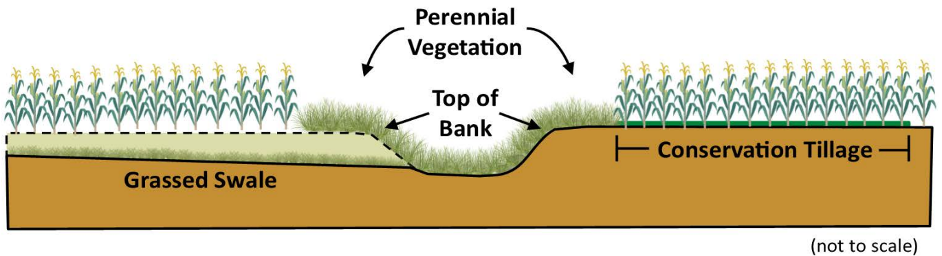
Figure 6: Cross Section view A, Alt Practice #4B
